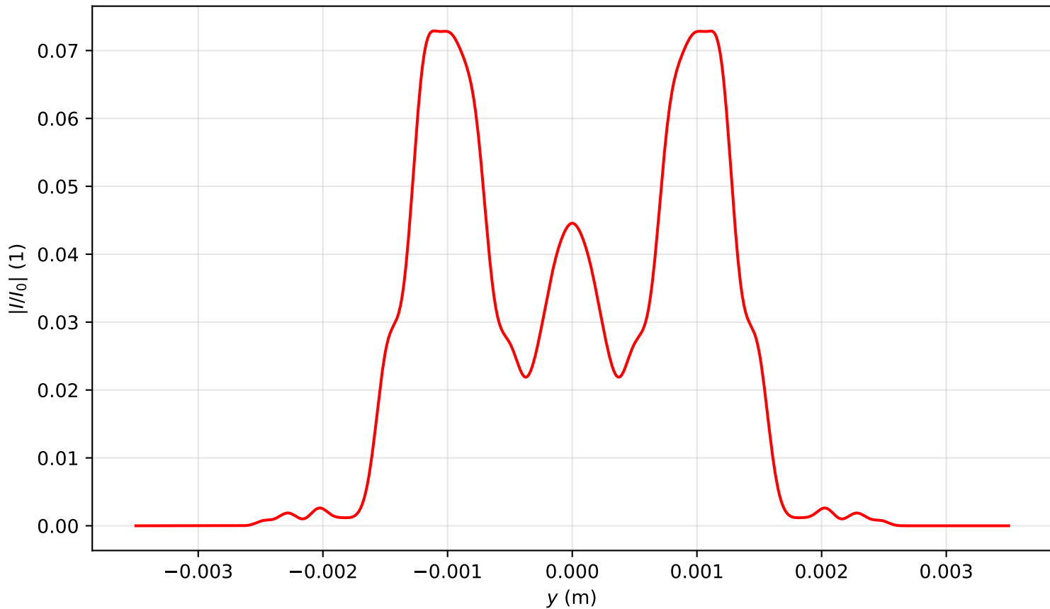
Intensity profile I(x=0, y, z=2.866)/I_0 , P_{in}=6.5P_{cr} , artificial time
